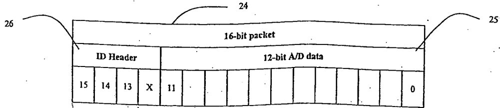
Figure 5a: Transmission Data Format
